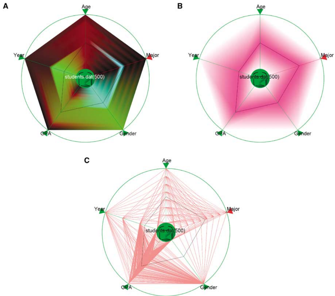
Figure 2 Sample DataRose visualization for a university student database of a computer science department. (A) Color histogram mode (high brightness equals high density). (B) Opacity bands mode. (C) Parallel coordinate mode.
