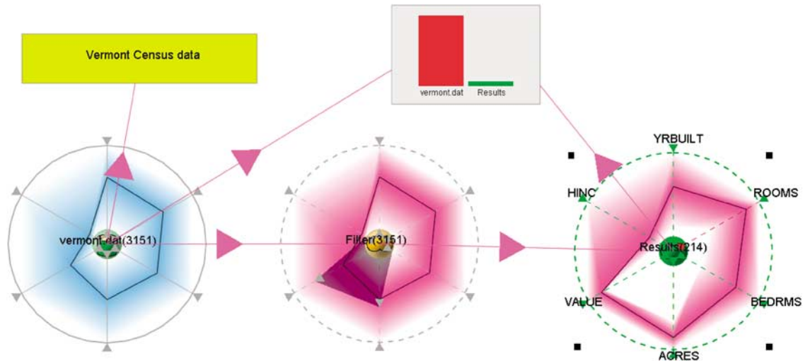
Figure 1 Sample house value and acreage vs number of rooms and owner income query in the DataMeadow.
