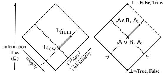
Fig. 8: Robust Declassification
