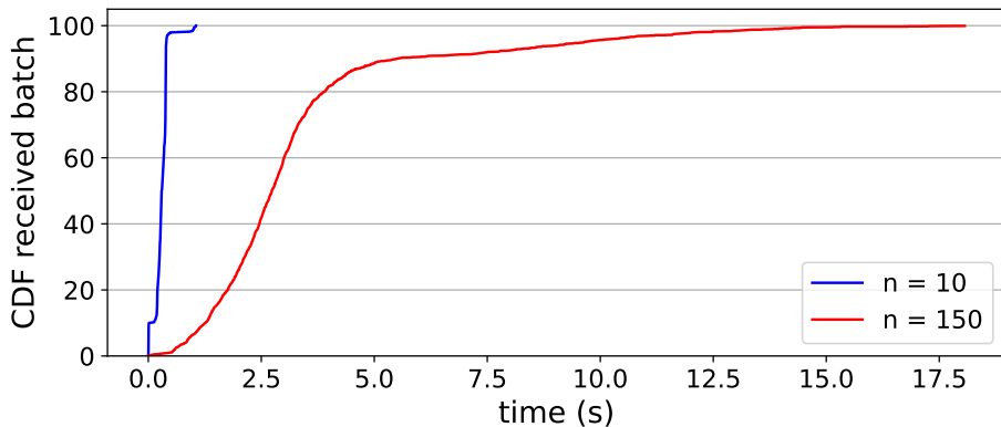
Plain all-to-all broadcast
