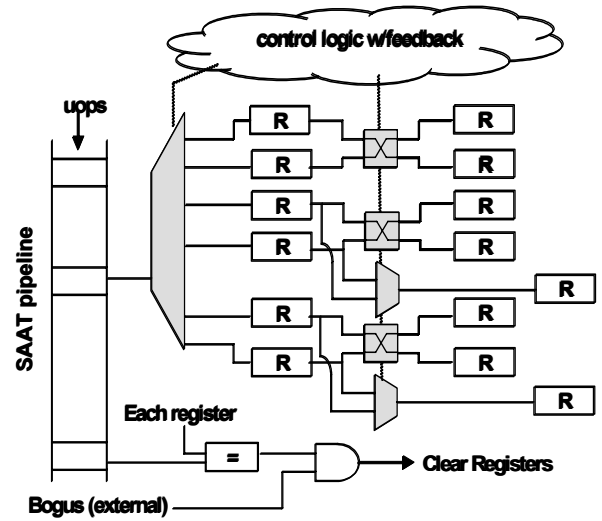
Figure 7. Pentium® 4 Memory Unit
