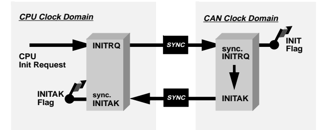
Figure 4-9 Initialization Request/Acknowledge Cycle
