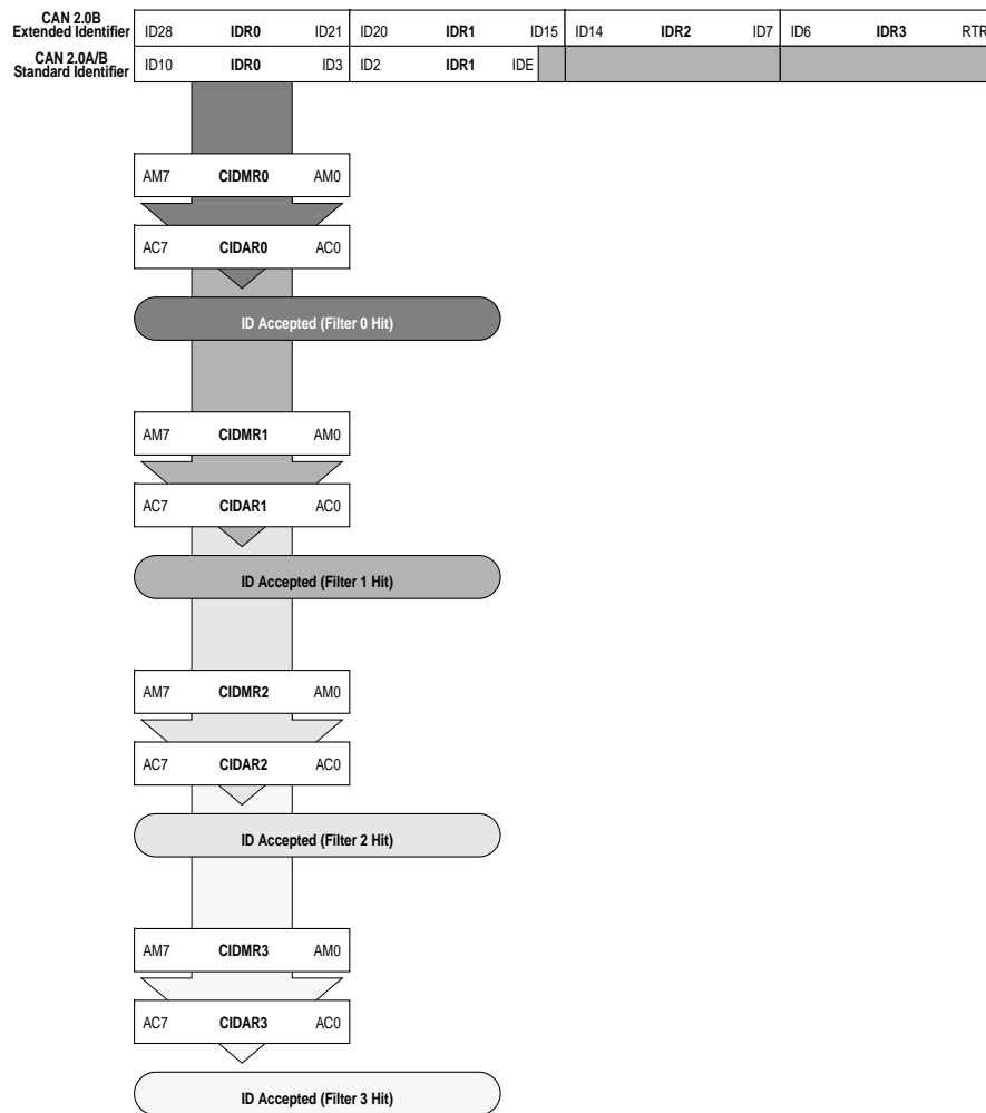
Figure 4-4 8-bit Maskable Identifier Acceptance Filters
