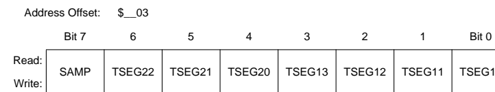
Figure 3-4 MSCAN Bus Timing Register 1 (CANBTR1)
