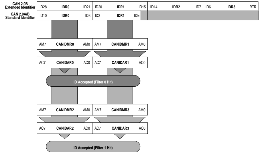
Figure 4-3 16-bit Maskable Identifier Acceptance Filters
