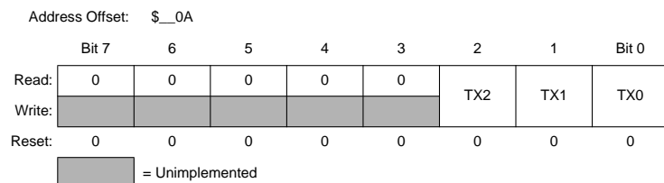
Figure 3-11 MSCAN Transmitter Flag Register (CANTBSEL)
