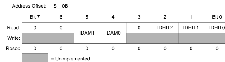
Figure 3-12 MSCAN Identifier Acceptance Control Register (CANIDAC)
