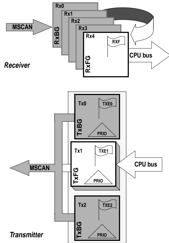
Figure 4-1 User Model for Message Buffer Organization
