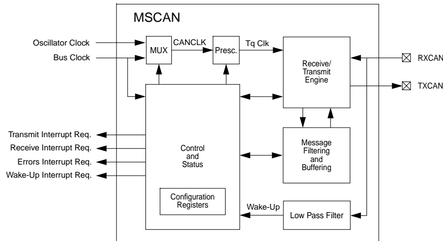
Figure 1-1 MSCAN Block Diagram
