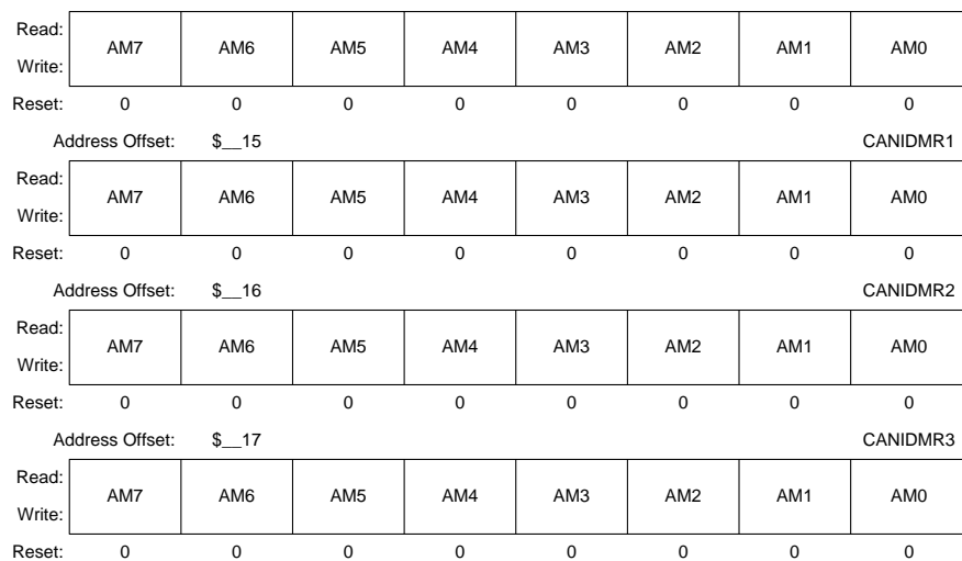
Figure 3-18 MSCAN Identifier Mask Registers (1st Bank)
