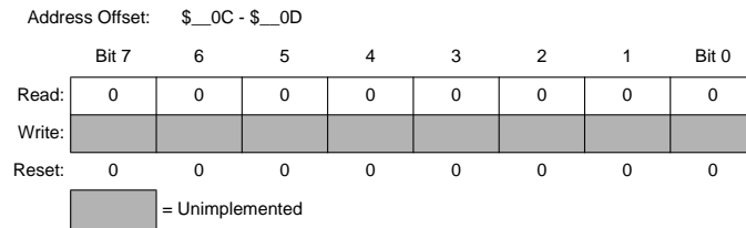
Figure 3-13 Reserved Registers
