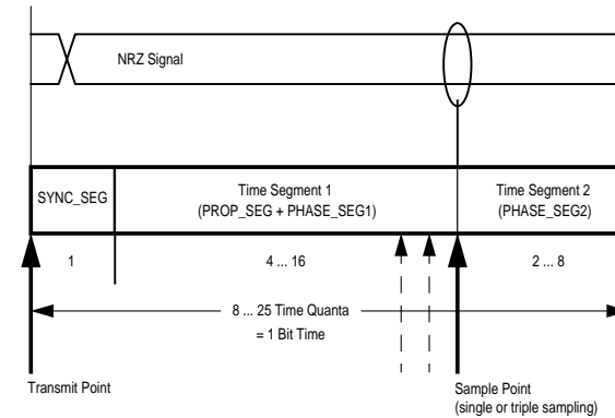
Figure 4-6 Segments within the Bit Time
