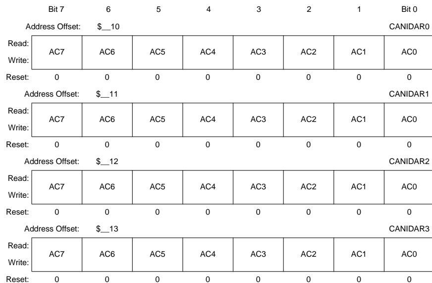
Figure 3-16 MSCAN Identifier Acceptance Registers (1st Bank)
