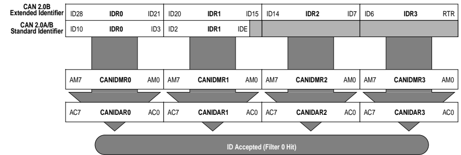
Figure 4-2 32-bit Maskable Identifier Acceptance Filter
