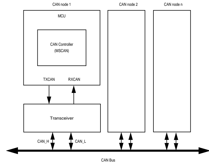
Figure 2-1 The CAN System
