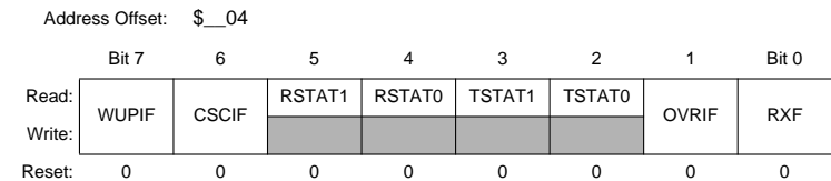
Figure 3-5 MSCAN Receiver Flag Register (CANRFLG)
