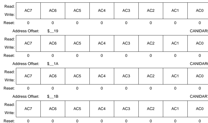
Figure 3-17 MSCAN Identifier Acceptance Registers (2nd Bank)
