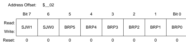
Figure 3-3 MSCAN Bus Timing Register 0 (CANBTR0)
