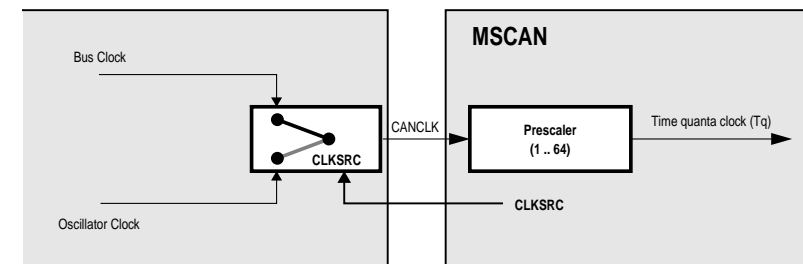
Figure 4-5 MSCAN Clocking Scheme
