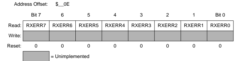
Figure 3-14 MSCAN Receive Error Counter Register (CANRXERR)
