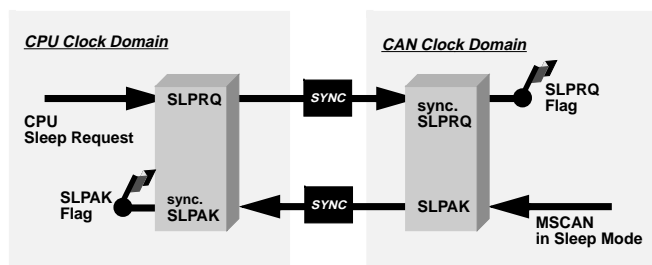
Figure 4-7 Sleep Request / Acknowledge Cycle
