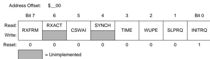
Figure 3-1 MSCAN Control 0 Register (CANCTL0)
