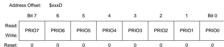
Figure 3-22 Transmit Buffer Priority Register (TBPR)
