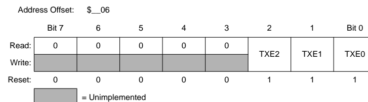
Figure 3-7 MSCAN Transmitter Flag Register (CANTFLG)
