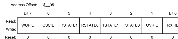
Figure 3-6 MSCAN Receiver Interrupt Enable Register (CANRIER)
