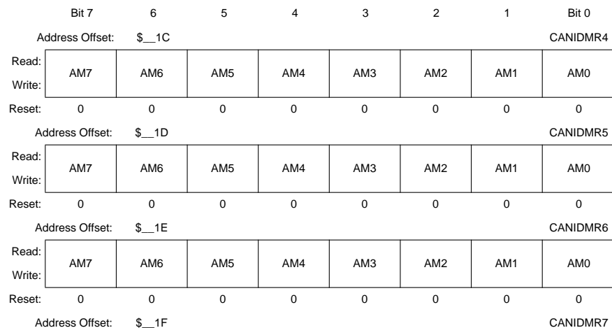
Figure 3-19 MSCAN Identifier Mask Registers (2nd Bank)
