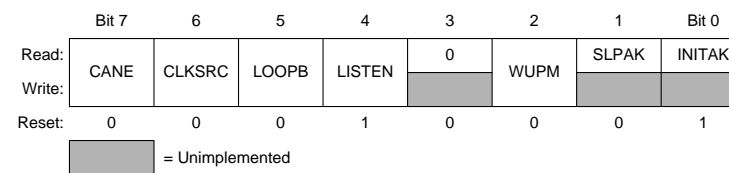
Figure 3-2 MSCAN Control 1 Register (CANCTL1)
