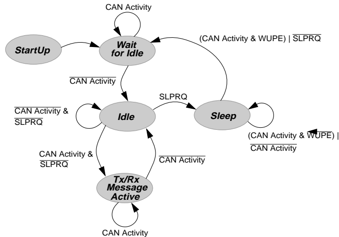
Figure 4-8 Simplified State Transitions for Entering/Leaving Sleep Mode
