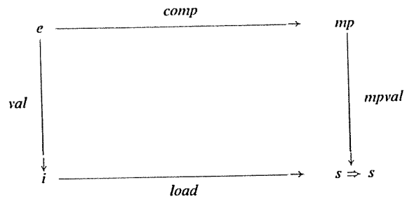
Fig. 2. Correctness of compilation. The condition is that this diagram commutes. The function load is load(i) = \lambda s.i :: s
