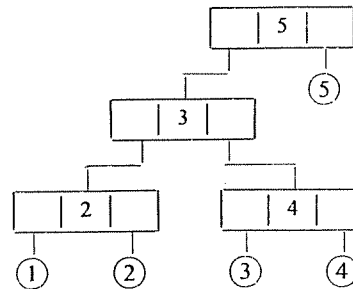
Fig. 1. Tree obtained in sorting the list (3, 5, 2, 1, 4) into the list (1, 2, 3, 4, 5)
