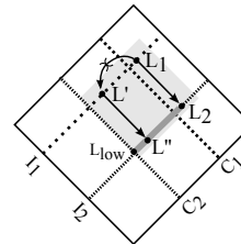
Fig. 11: Bounded endorsement and robust declassification.
