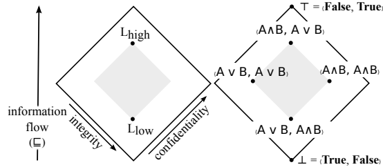
Fig. 7: Bounded Downgrading
