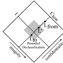
Fig. 10: Bounded and robust declassification.
