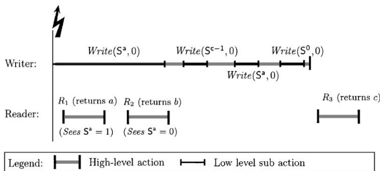
FIG. 3. The danger of using a while loop.
