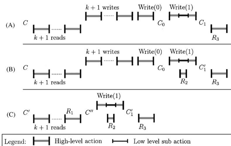
FIG. 1. The runs constructed in the proof of Theorem 1.
