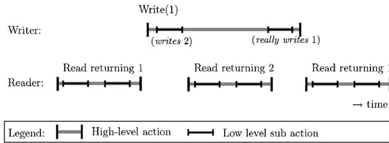
FIG. 2. Repeating actions does not make an object 1-stabilizing.
