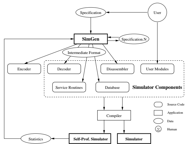
Figure 2 - SIMGEN Overview
