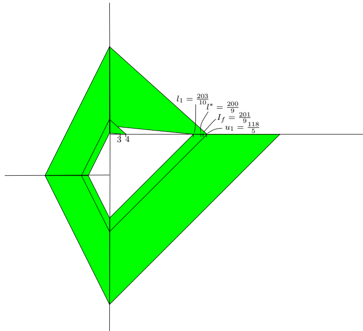
Fig. 16. Simulation of reachability for x_f = \frac{201}{9} .
