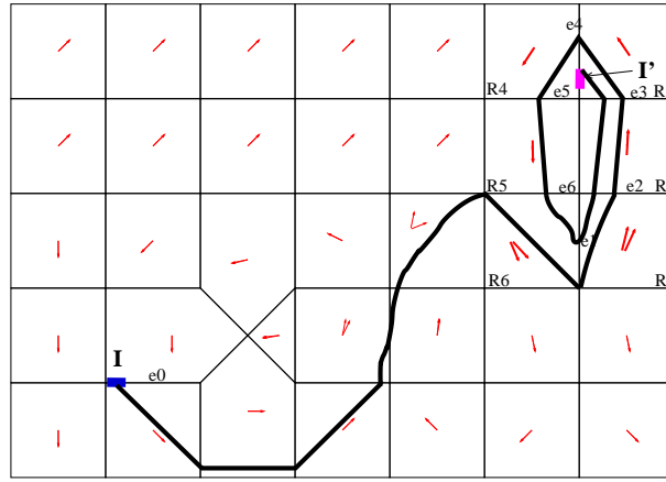
Fig. 1. An SPDI and its trajectory segment.
