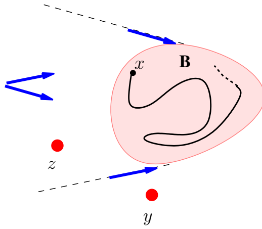
Fig. 6. Example 9: Controllability kernel.
