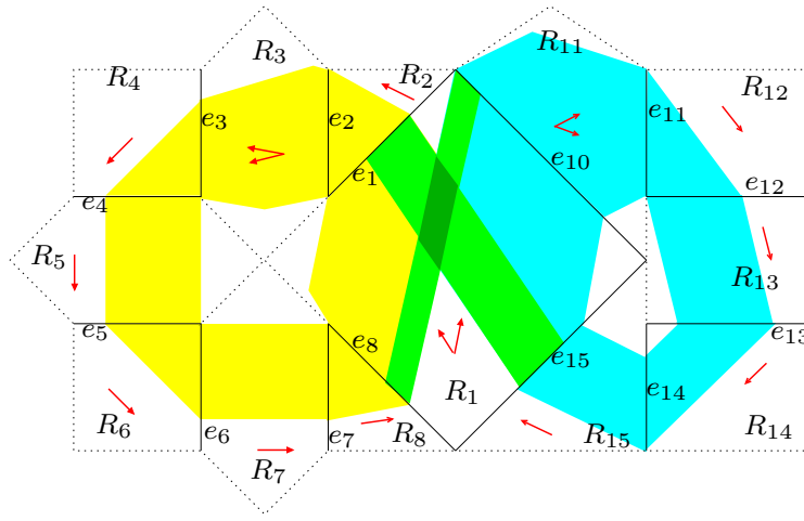
Fig. 9. Another SPDI and its “phase-portrait”.
