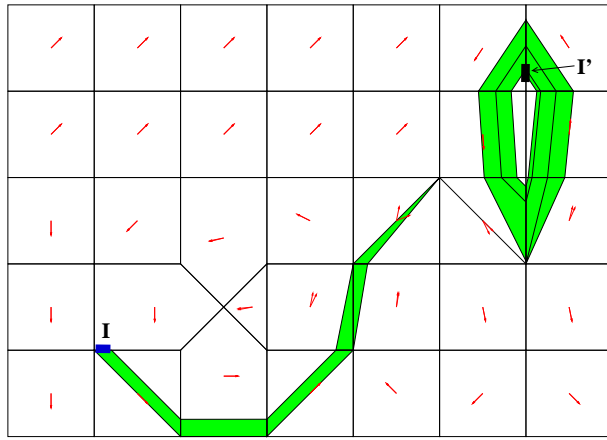
Fig. 2. Reachability analysis.
