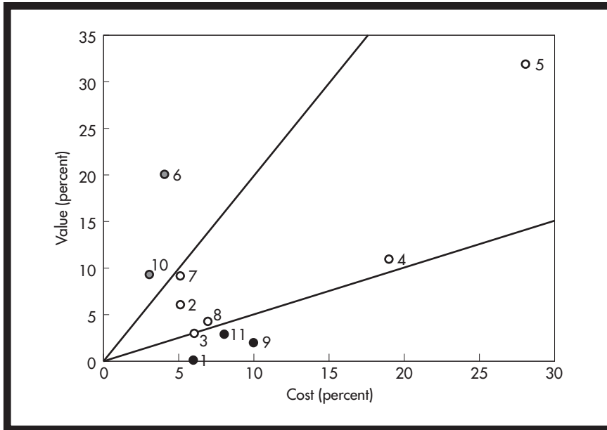
Figure 7. Cost-value diagram depicting the PMR project requirements.
