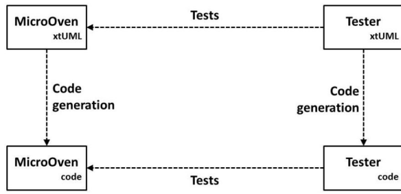
Fig. 3. The Tester-model can be reused at code level through code generation.
