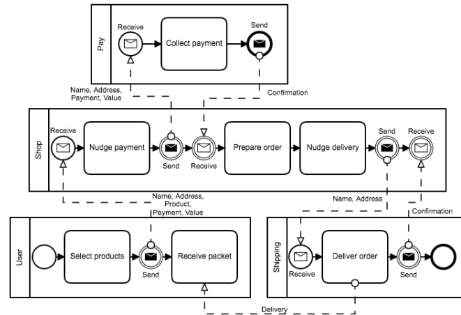
Fig. 1: Traditional Shopping Process in Business Process Modeling Notation [Ob11]
