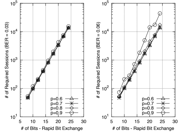
FIGURE 6. Expected number of required eavesdropped sessions for noisy communication channel as the required success probability p varies. The left and right panels show the result for BER = 0.03 and BER = 0.06 respectively, with k = n , d = 2^n .
