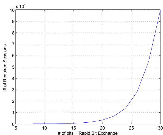
FIGURE 3. Expected number of required sessions for ideal communication channel ( BER = 0.0 ) for as n increases, with k = n , d = 2^n .
