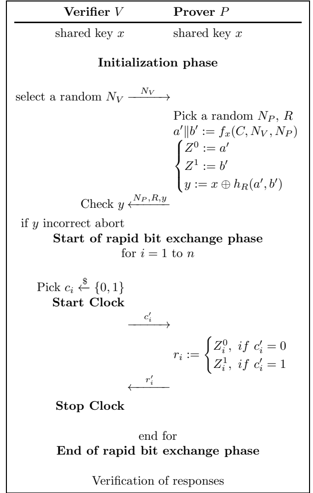
FIGURE 8. The general view of the distance bounding protocols proposed in [10, 7, 8, 9] modified with the proposed countermeasure secure against terrorist fraud attacks.
