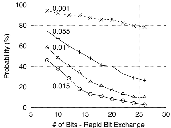
FIGURE 4. Adversary's success probability for noisy communication channel as n increases, with k = n , d = 2^n .
