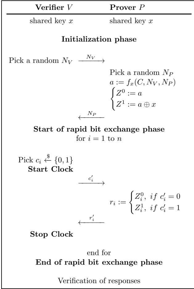
FIGURE 1. A general view of the distance bounding protocols proposed in [10, 7, 8, 9]
