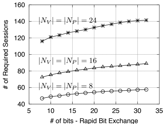
FIGURE 2. Expected number of required sessions for ideal communication channel ( BER = 0.0 ) for various nonce lengths m as the number of rounds n and the key length k = n increase. Note that the number of sessions is scaled down by 10 and 100 for m = 16 and m = 24 respectively.
