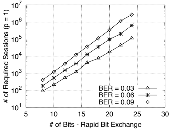
FIGURE 7. Expected number of required eavesdropped sessions for noisy communication channel ( BER = \{0.03, 0.06, 0.09\} ) with k = n , d = 2^n .
