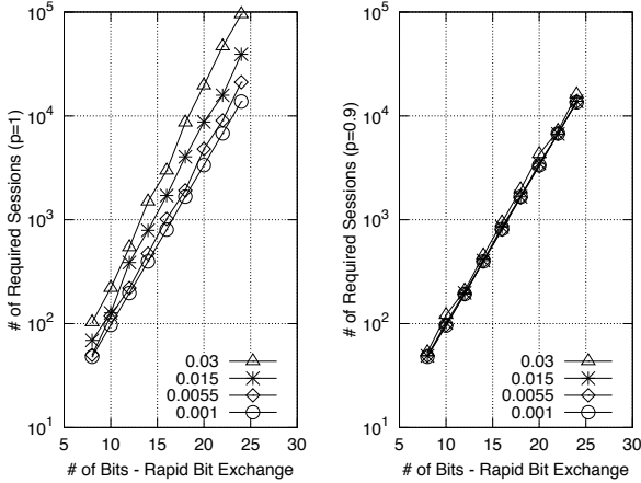
FIGURE 5. Expected number of eavesdropped sessions required for noisy communication channel with k = n , d = 2^n as the BER varies. The left and right panels show the result for success probability p = 1 and p = 0.9 respectively.
