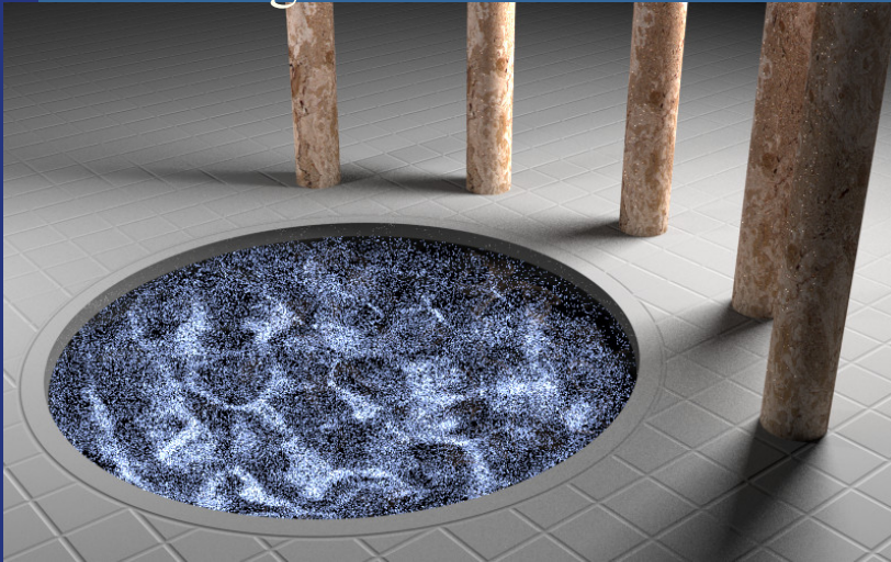
Path tracing
