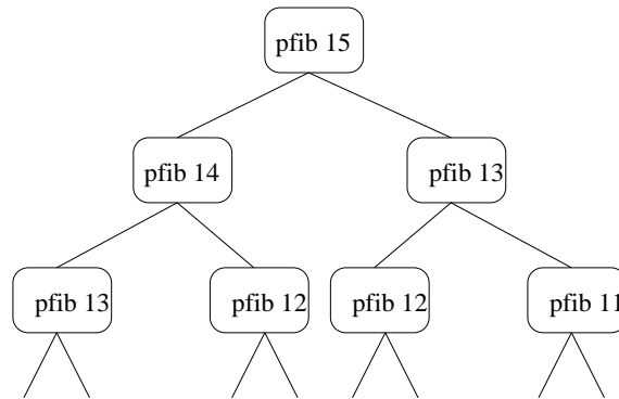
Fig. 1. p fib Divide-and-conquer Process Diagram
