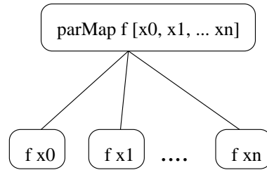
Fig. 2. parMap Process Diagram
