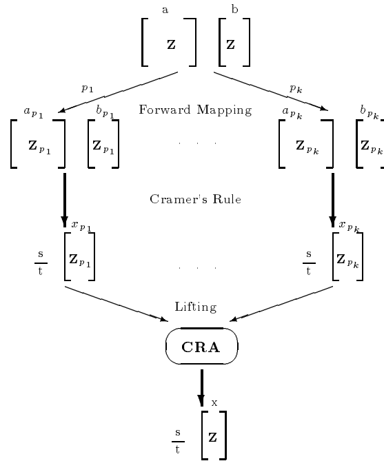
Fig. 8. Structure of the LinSolv algorithm
