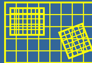
Hierarchical grid
