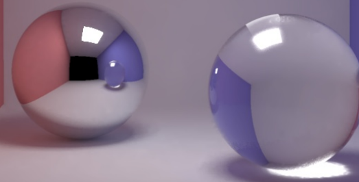
Global Illumination
