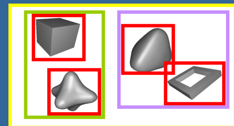
Hierarchical grid
