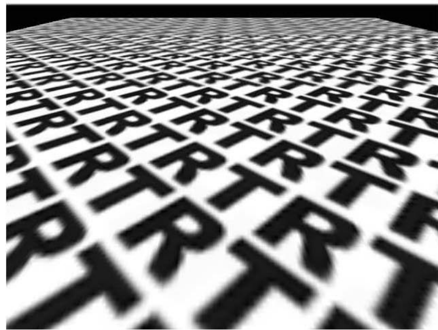
pixel space
