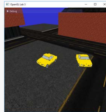
Animation
