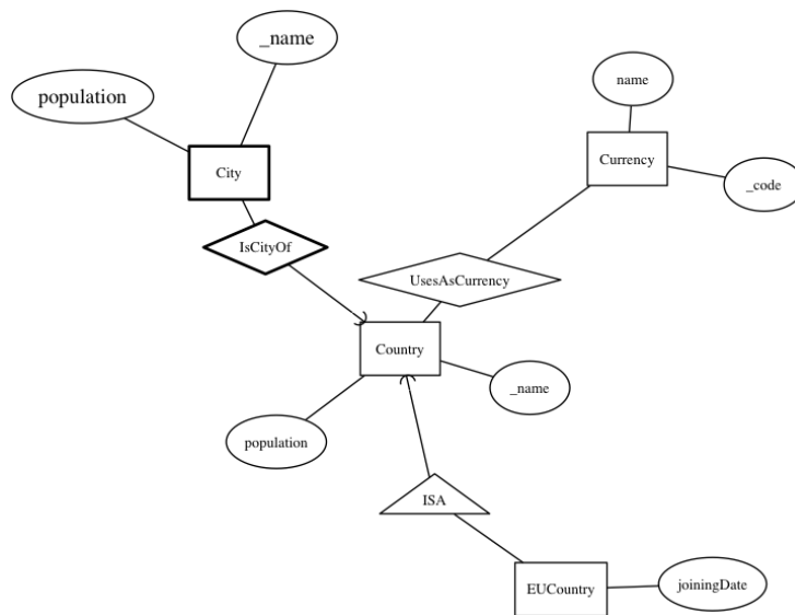
Figure 2: An E-R diagram generated from the Query Converter qconv. Weak entities and relationships have thick borders.
