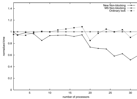
(c) Quick-sort on SUN Starfire
