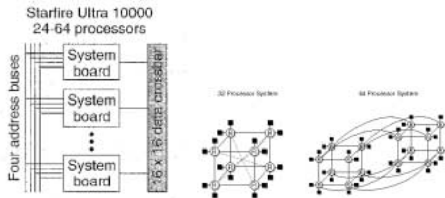
(a) The architecture of the SUN Enterprise 10000
