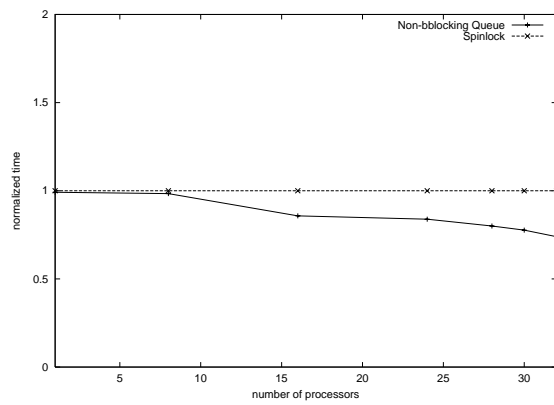
(b) Radiosity
