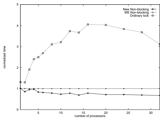
(a) Quick-sort
