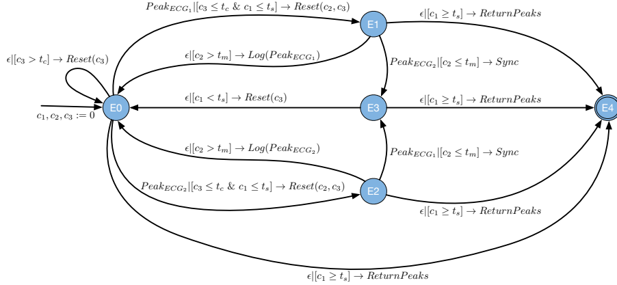
Figure 7: Heart based timed automaton.
