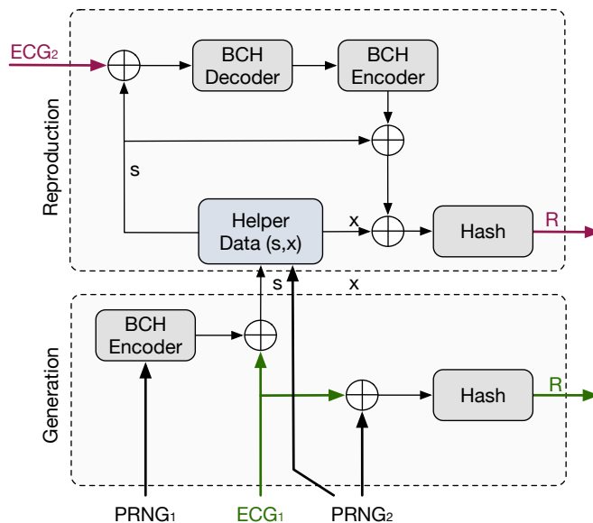
Figure 5: Fuzzy extractor.
