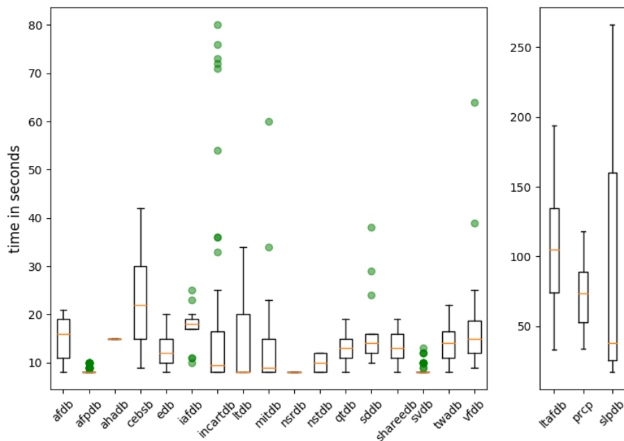
Figure 8: Time needed to generate a 32-bit token.
