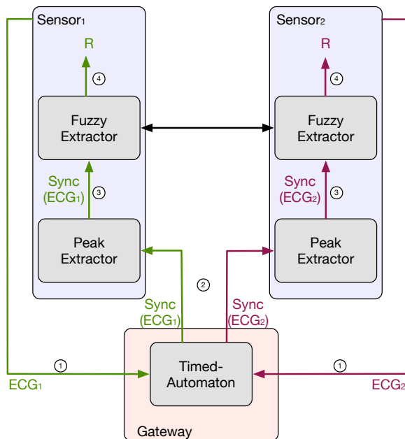
Figure 11: System model using both a timed automaton and a fuzzy extractor.
