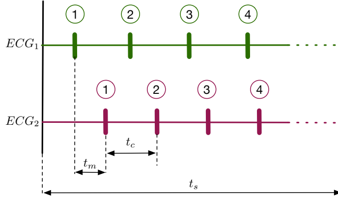
Figure 6: Time-checks used in the timed automaton.
