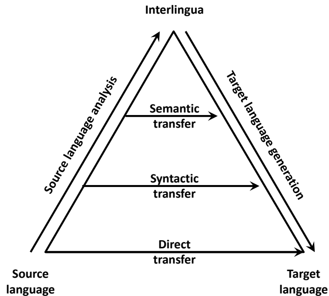
Figure 1: The Vauquois translation triangle
