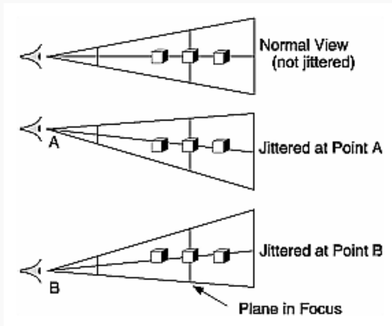
Figure 10-3 : Jittered Viewing Volume for Depth-of-Field Effects
