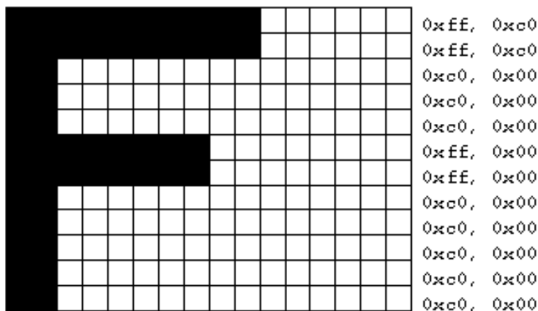
Figure 8-1 : Bitmapped F and Its Data
