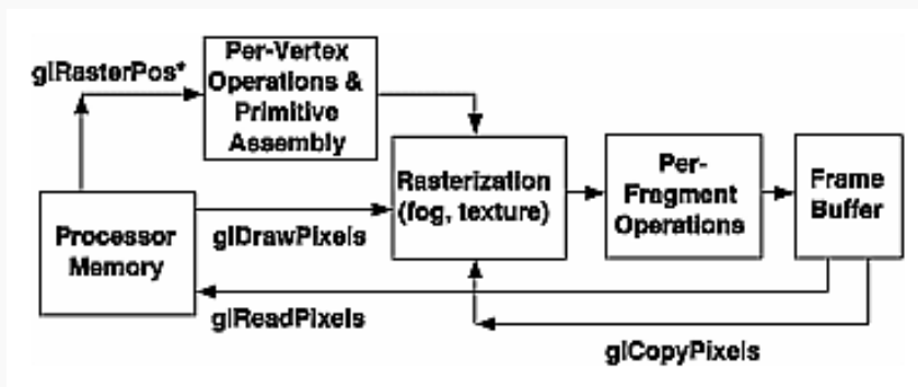
Figure 8-3 : Simplistic Diagram of Pixel Data Flow
