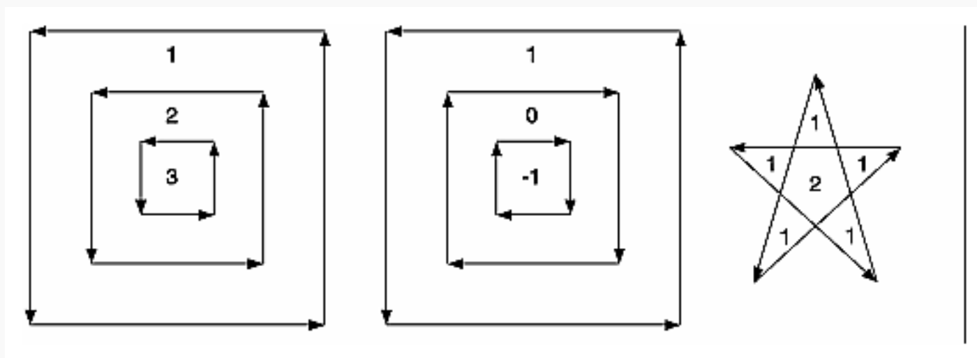
Figure 11-2 : Winding Numbers for Sample Contours
