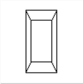
Figure 3-3 : Transformed Cube
