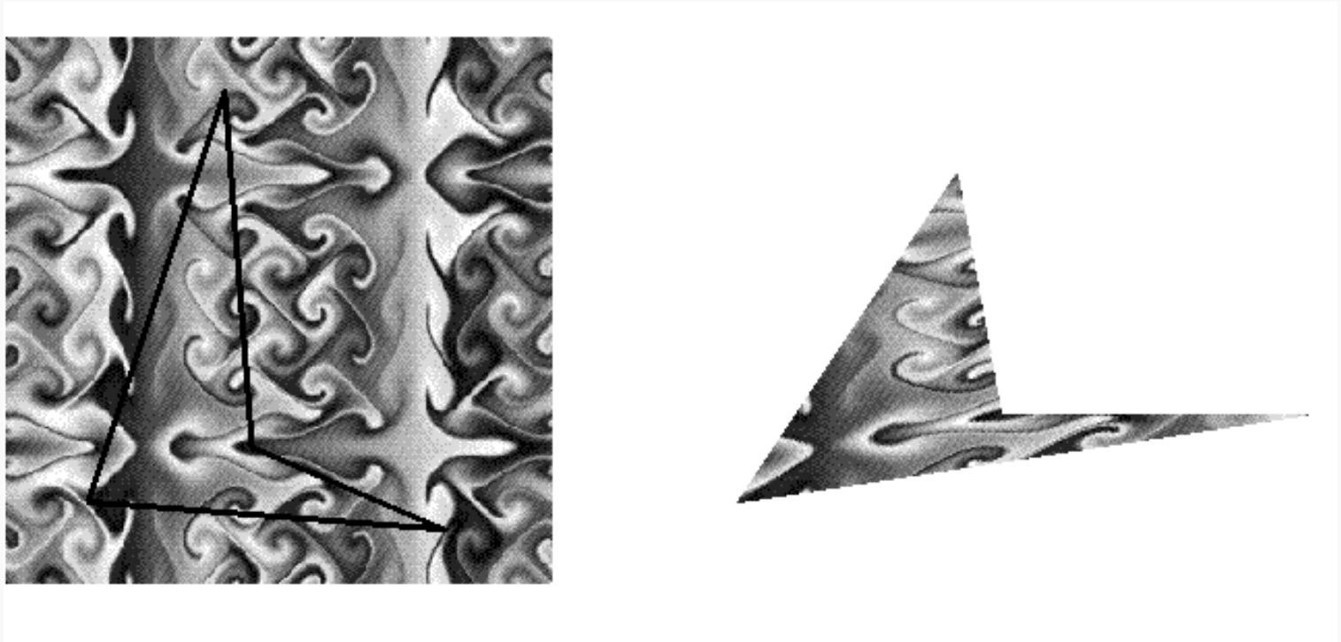
Figure 9-1 : Texture-Mapping Process
