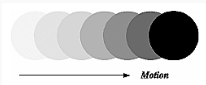
Figure 10-2 : Motion-Blurred Object
