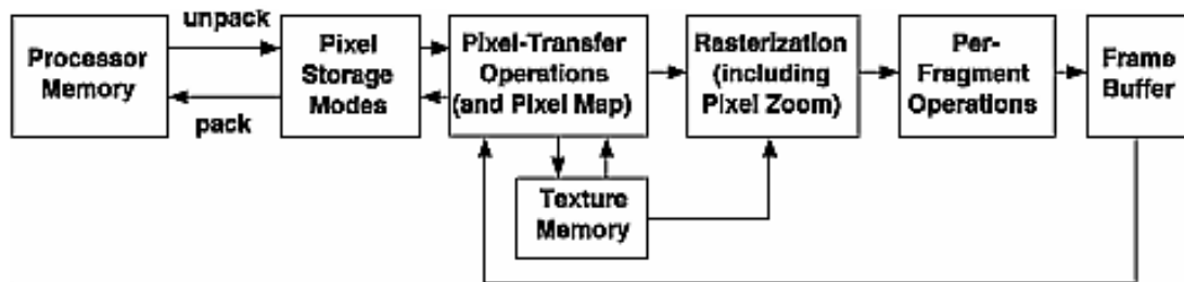
Figure 8-4 : Imaging Pipeline
