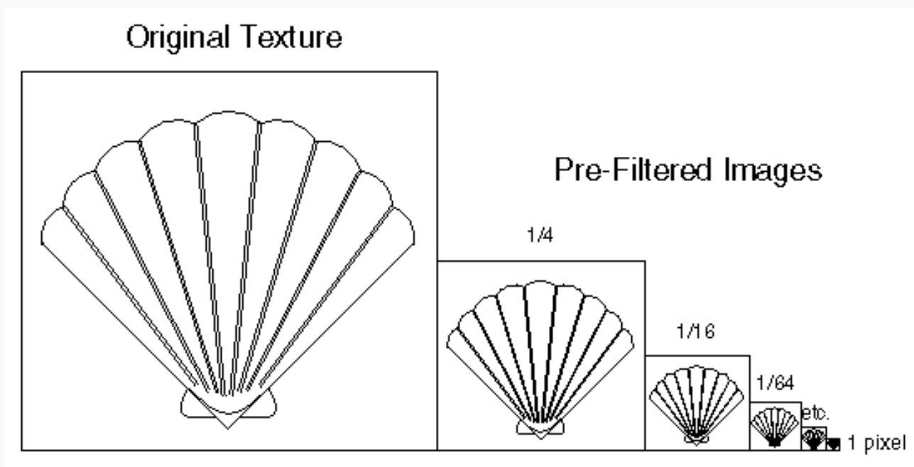
Figure 9-4 : Mipmaps
