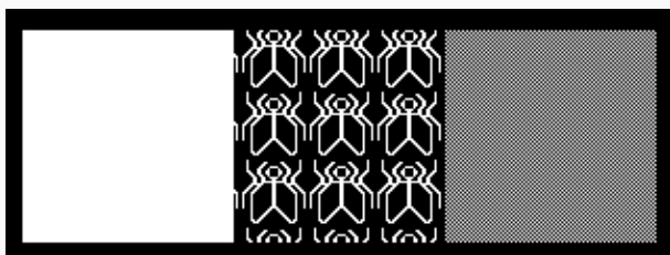
Figure 2-11 : Stippled Polygons
