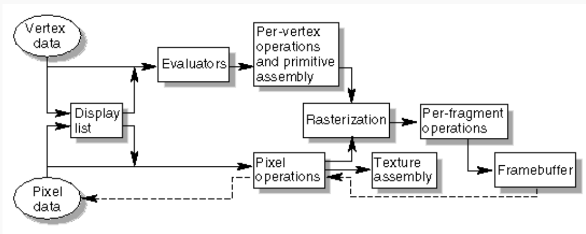
Figure 1-2 : Order of Operations
