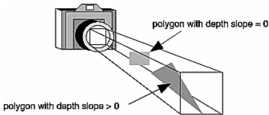
Figure 6-5 : Polygons and Their Depth Slopes
