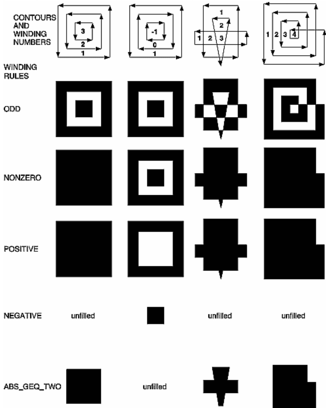
Figure 11-3 : How Winding Rules Define Interiors
