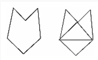
Figure 2-12 : Subdividing a Nonconvex Polygon
