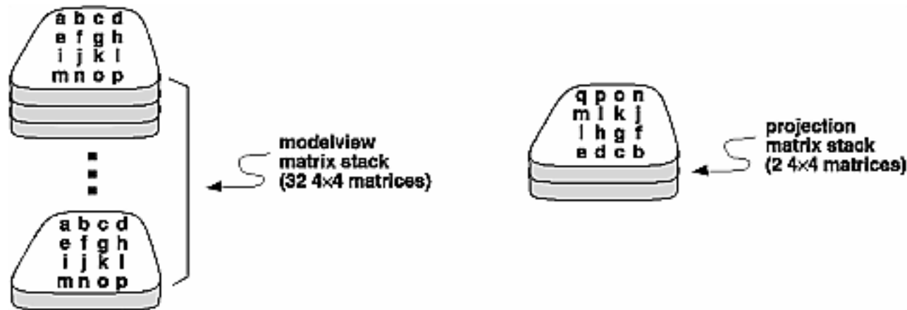
Figure 3-20 : Modelview and Projection Matrix Stacks
