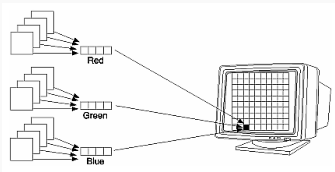
Figure 4-2 : RGB Values from the Bitplanes
