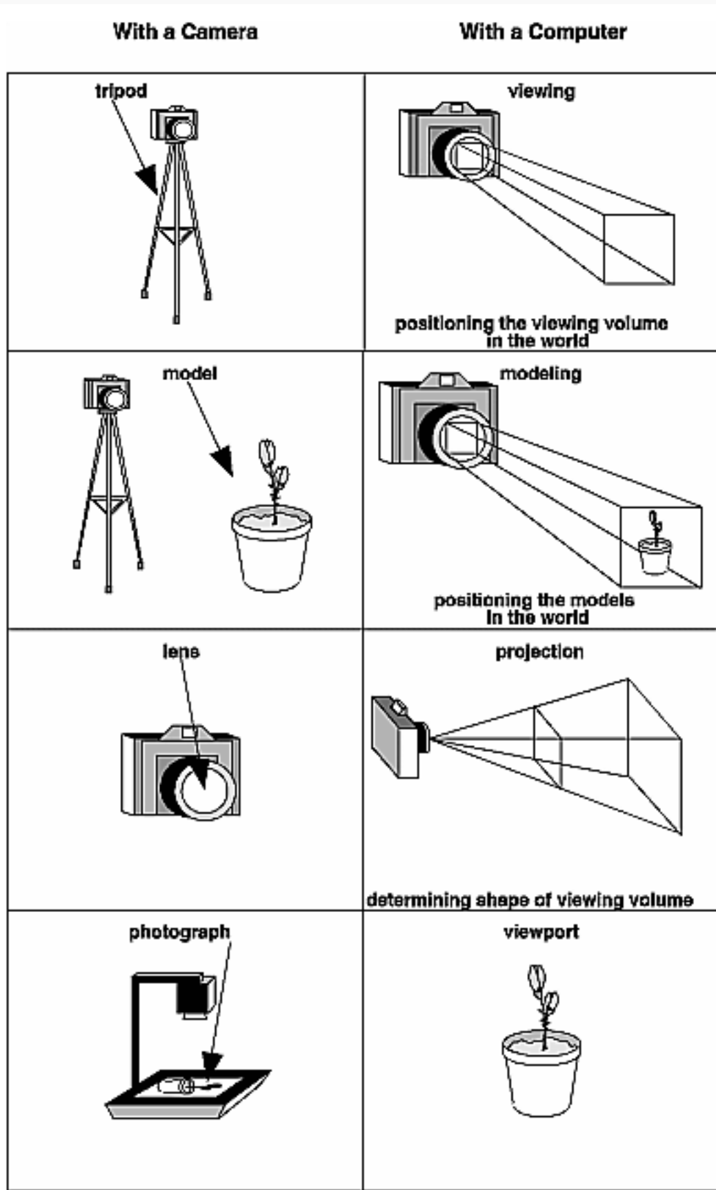
Figure 3-1 : The Camera Analogy
