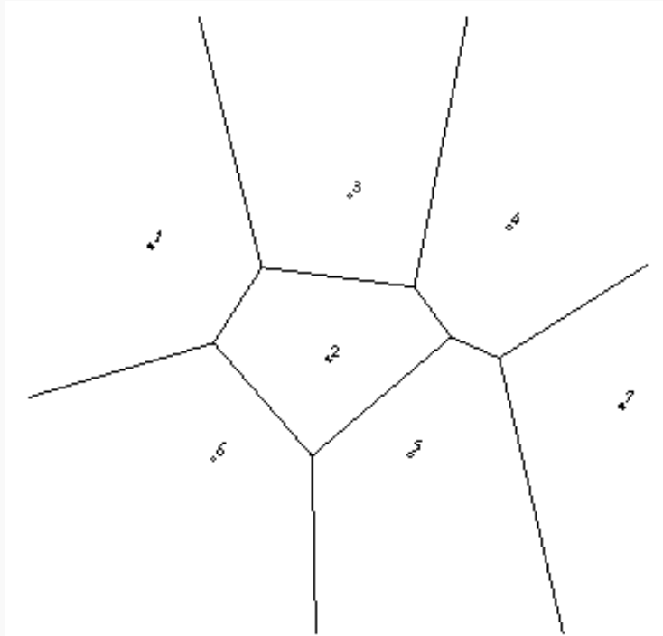
Figure 14-3 : Dirichlet Domains
