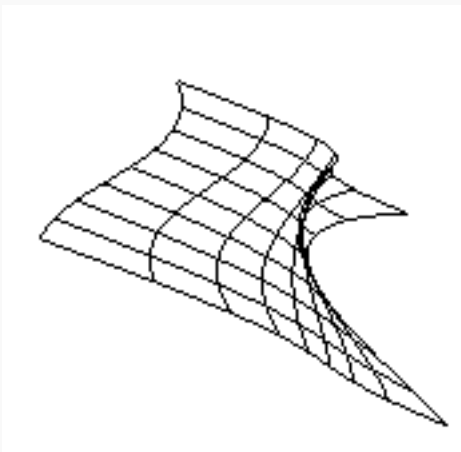
Figure 12-2 : Bézier Surface
