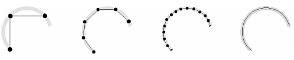
Figure 2-5 : Approximating Curves
