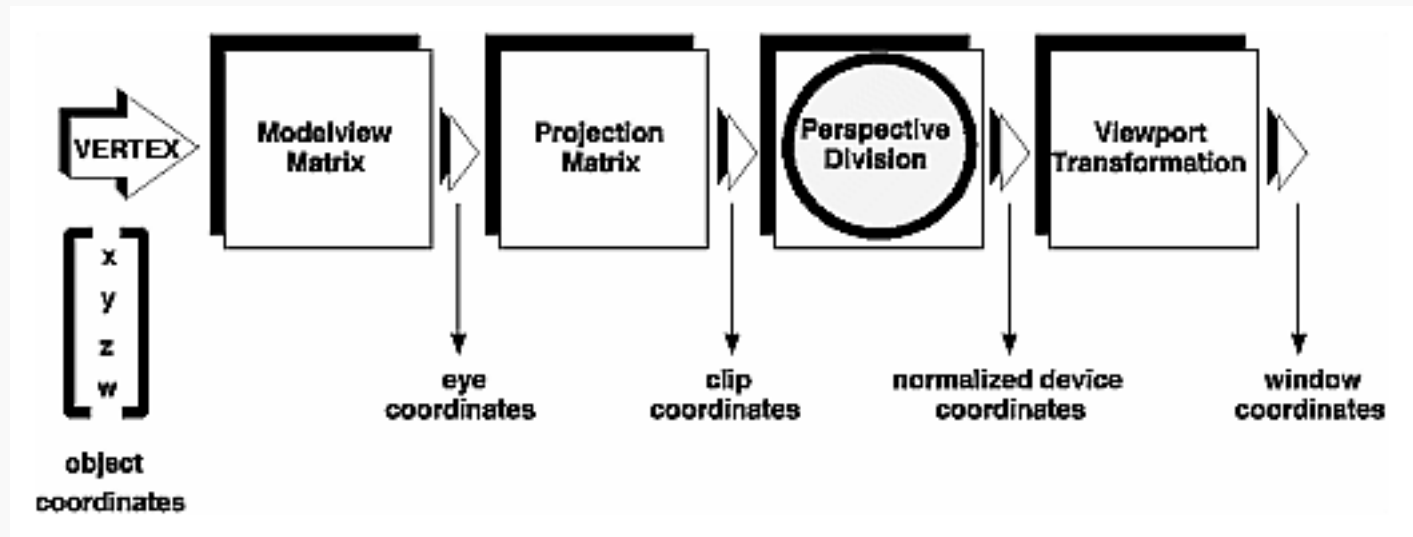
Figure 3-2 : Stages of Vertex Transformation
