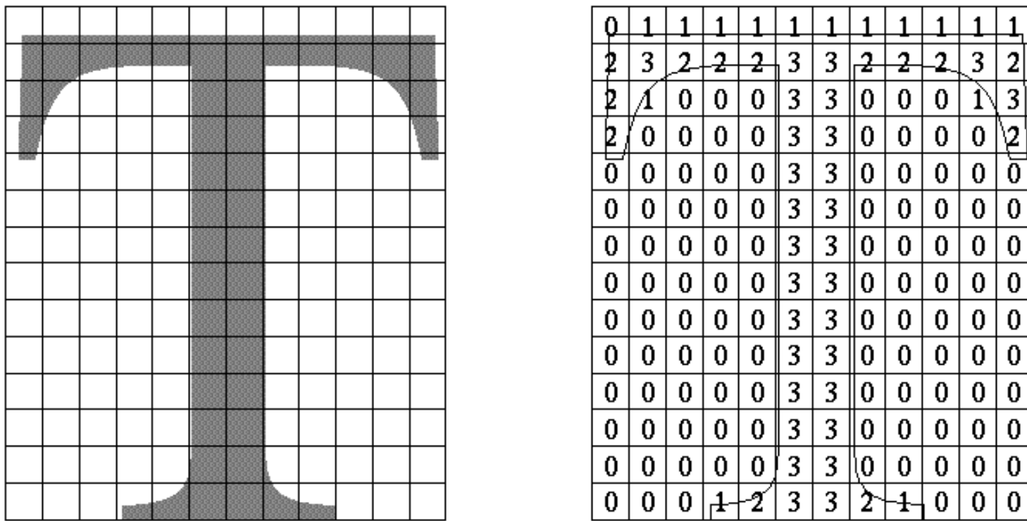
Figure 14-1 : Antialiased Characters
