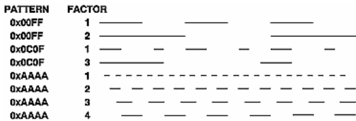
Figure 2-8 : Stippled Lines
