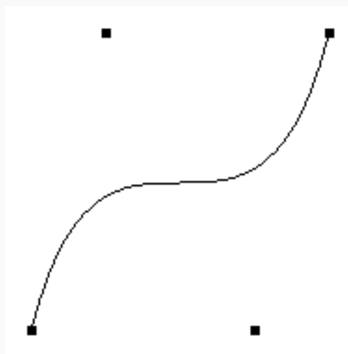
Figure 12-1 : Bézier Curve
