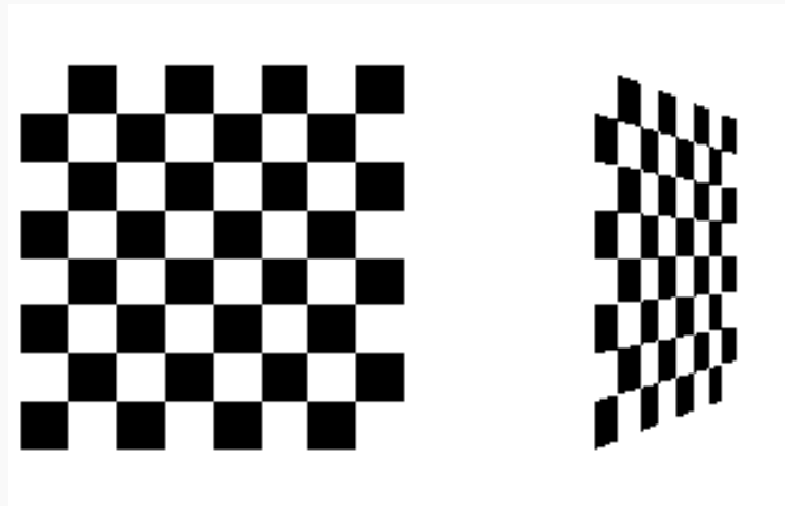
Figure 9-2 : Texture-Mapped Squares
