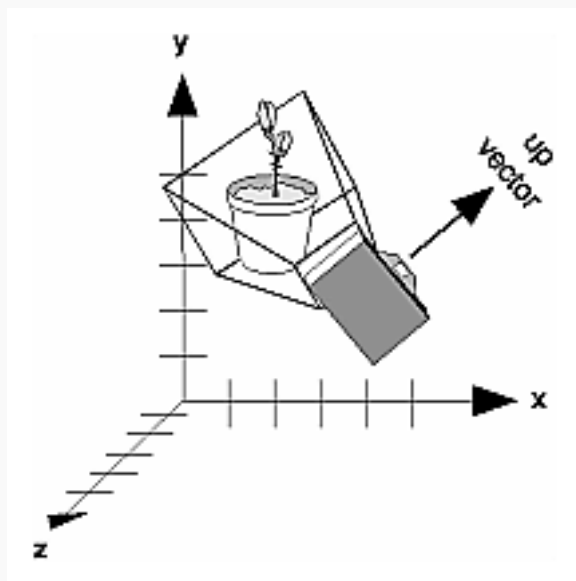
Figure 3-12 : Using gluLookAt()
