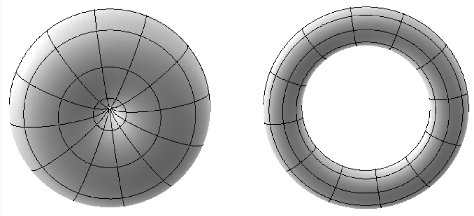
Figure 9-6 : Texture-Map Distortion
