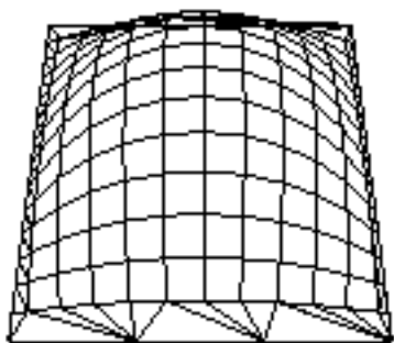
Figure 12-4 : NURBS Surface
