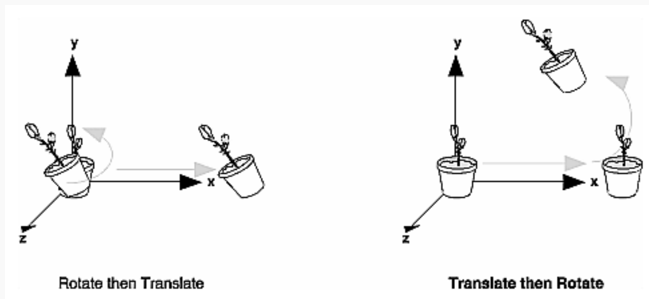
Figure 3-4 : Rotating First or Translating First
