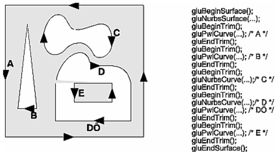
Figure 12-5 : Parametric Trimming Curves
