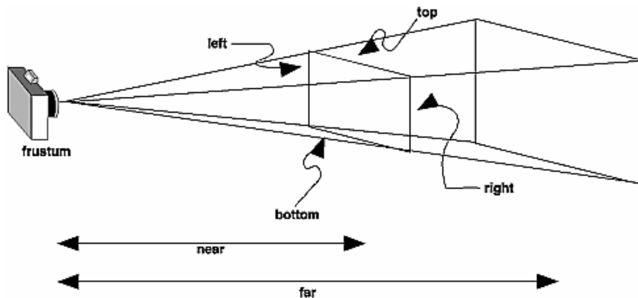
Figure 3-13 : Perspective Viewing Volume Specified by glFrustum()
